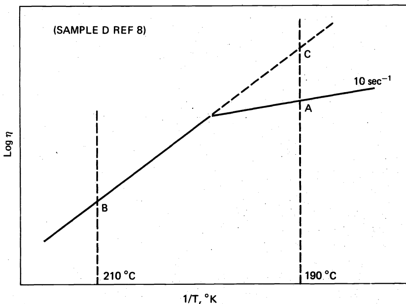
Fig. 1. Viscosity at 10 \text{ sec}^{-1} vs. Reciprocal Absolute Temperature for Sample D, Ref. (8).
