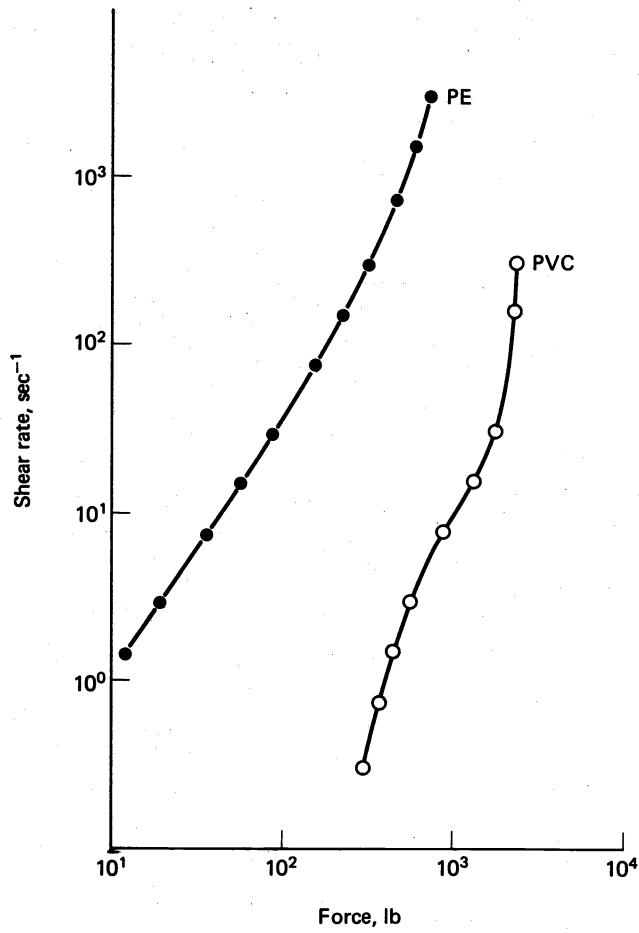
Fig. 7. Flow Curves for a PVC Compound and High Density Polyethylene at 180°C ( L/D = 39.4 ) - Bars Represent Extreme Values.
