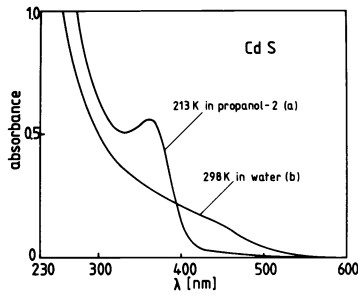
Fig.3 Spectra of colloidal CdS at different particle size. The particles in water were produced by precipitation of CdS in the presence of 6 \times 10^{-3}M colloidal SiO 2 (Ludox HS30 from Dupont; particle size: 13 nm). They have a diameter of about 3 nm. The smaller particles in propanol-2 were produced without a carrier
