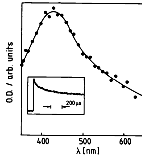
Fig.12 Absorption spectrum of trapped holes in \text{TiO}_2
