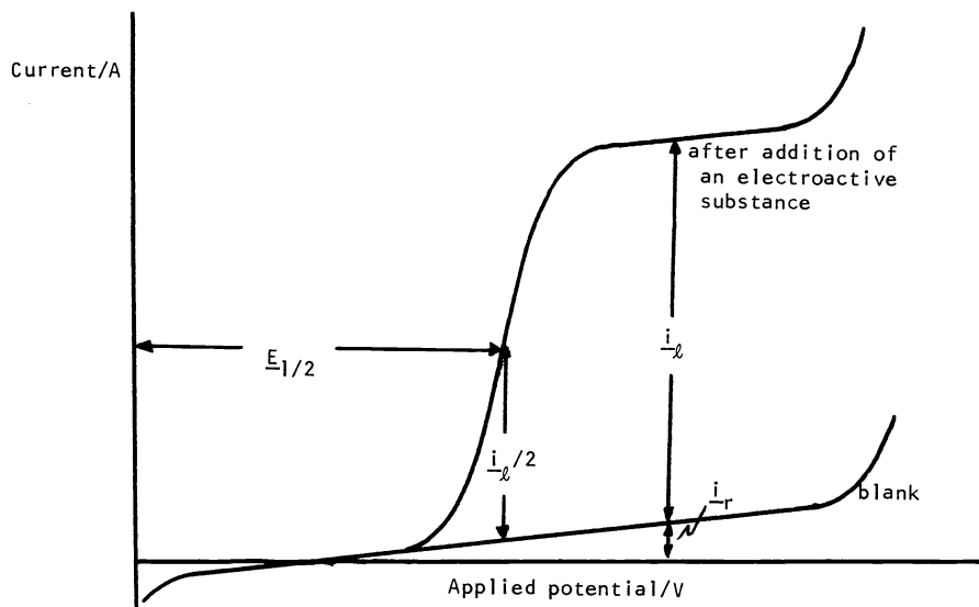
Fig. 1. Idealized polarogram, illustrating the limiting current i_l , the residual current i_r , and the half-wave potential E_{1/2} .
