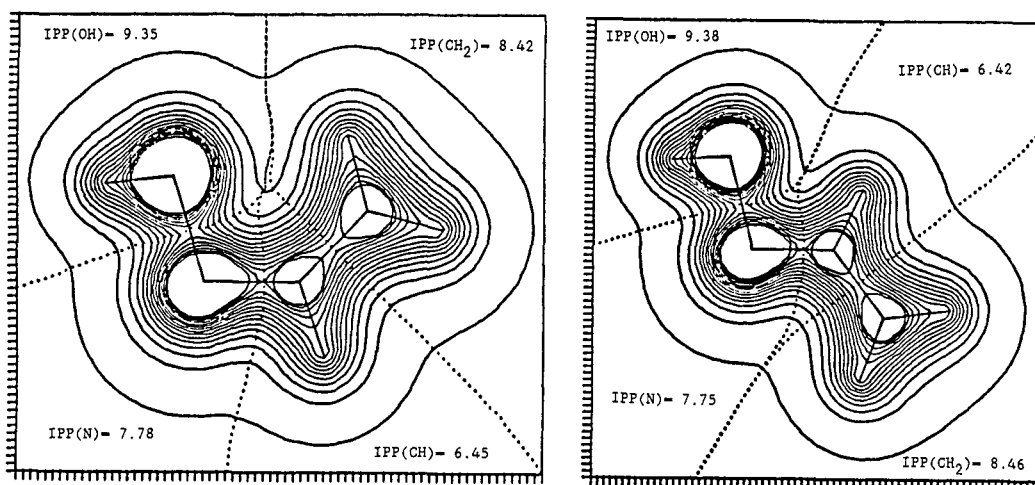
Fig. 2. Contour diagrams of the projected electron density functions of the syn ( 4 , left) and the anti ( 5 , right) carbanions of acetaldoxime. Contour levels start at 0.005 \text{ e a.u.}^{-2} with a level spacing of 0.05 .
